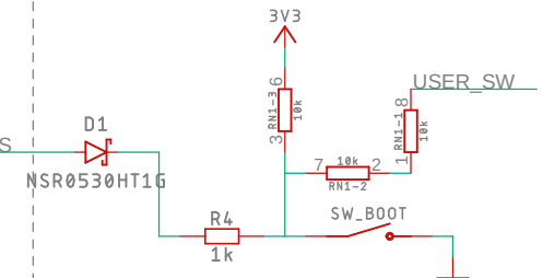
Combined USB boot & user switch
