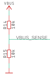
Vbus sense voltage divider
