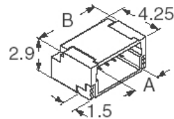
Male PCB Header
