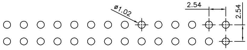
Recommended P.C.B. Layout (Top Side) (PCB Board Tolerance ±0.05)
